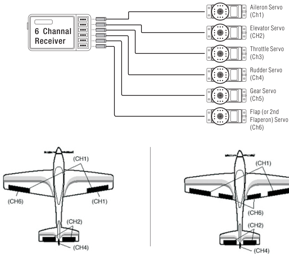
Flaperon Mode (Dual Aileron Servos CH1&6)
